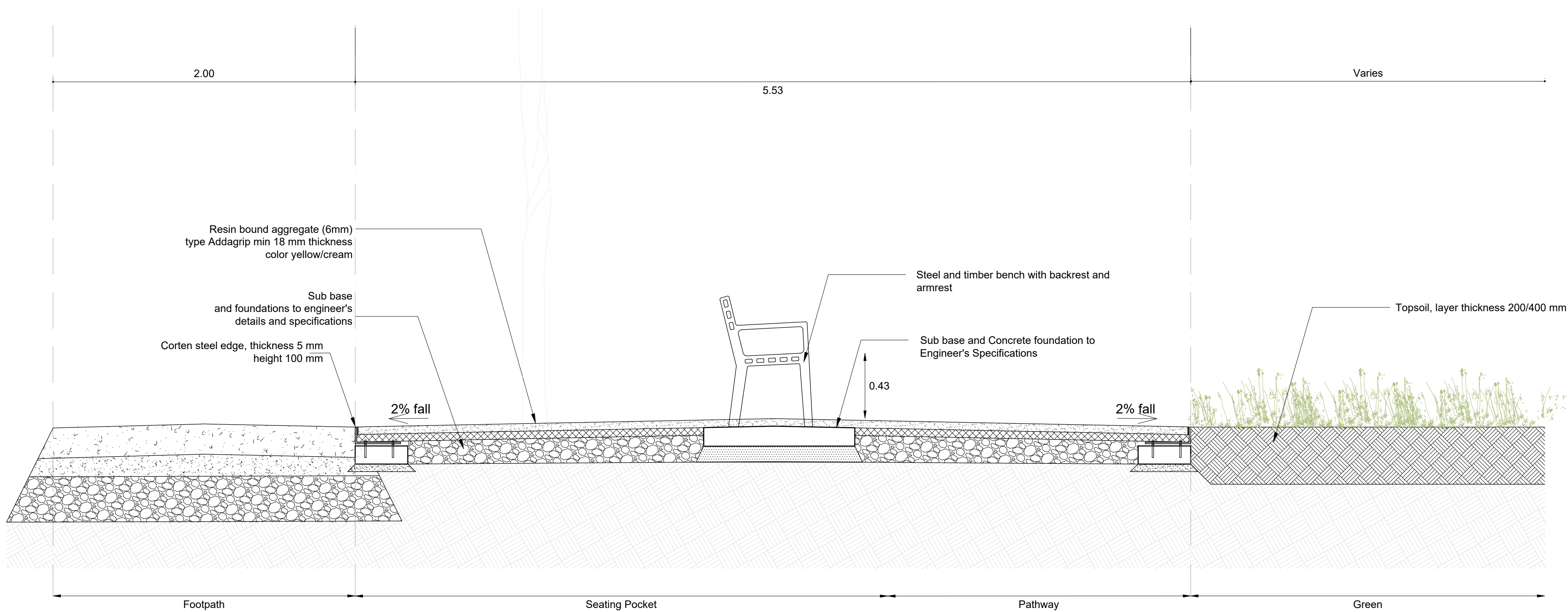
1 SEATING AREA TYPICAL PLAN AND CROSS SECTION
